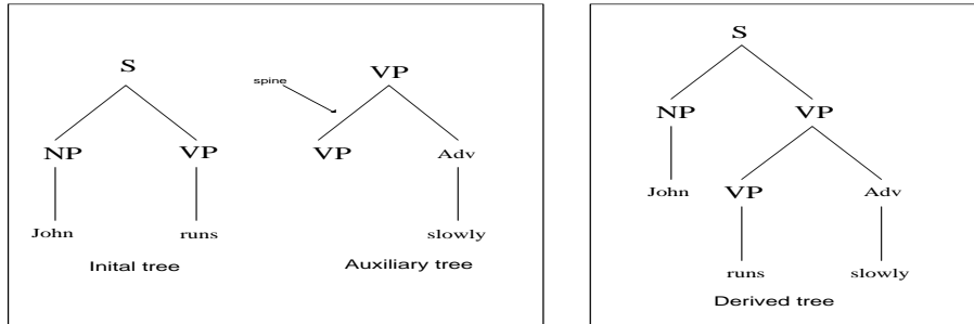
Figure 1. Adjunction operation
